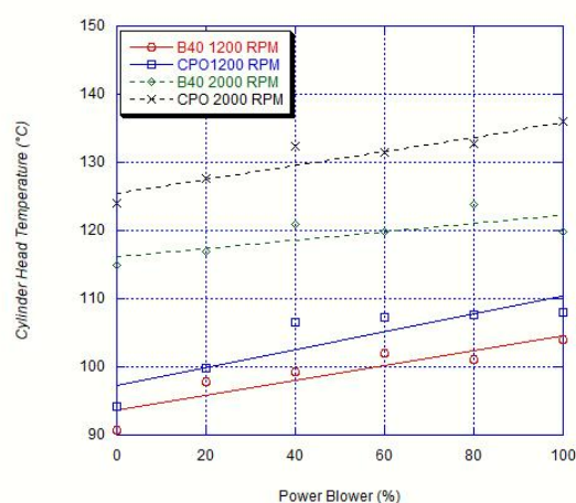
Fig. 2. Cylinder head temperature graph at 1200 and 2000 RPM
